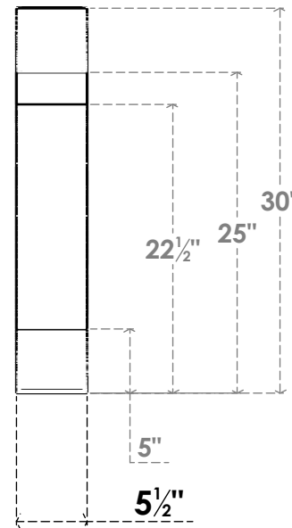
FRONT PROFILE
